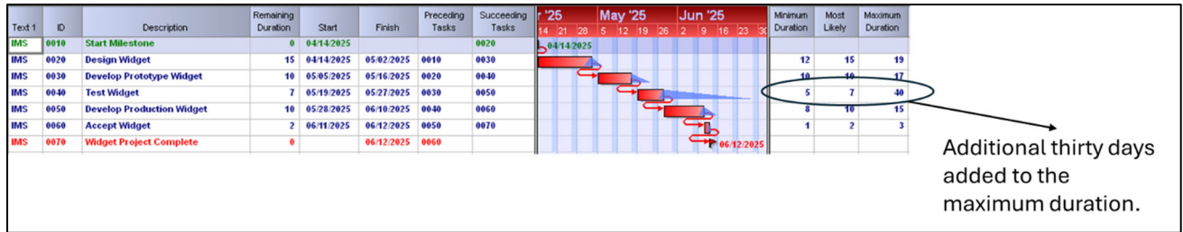
Figure 10.3.2-5 Example SRA Input - Incorrectly modeling a discrete risk in a worst case duration estimate
