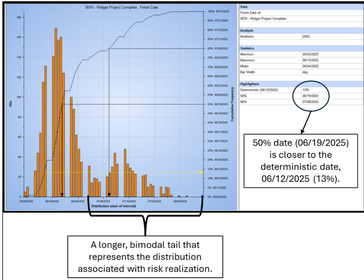
Figure 10.3.2-4 Histogram SRA data when discrete risk is properly modeled as an SRA input
