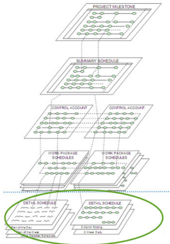
Figure 13.4-3 Example of Schedule Hierarchy
