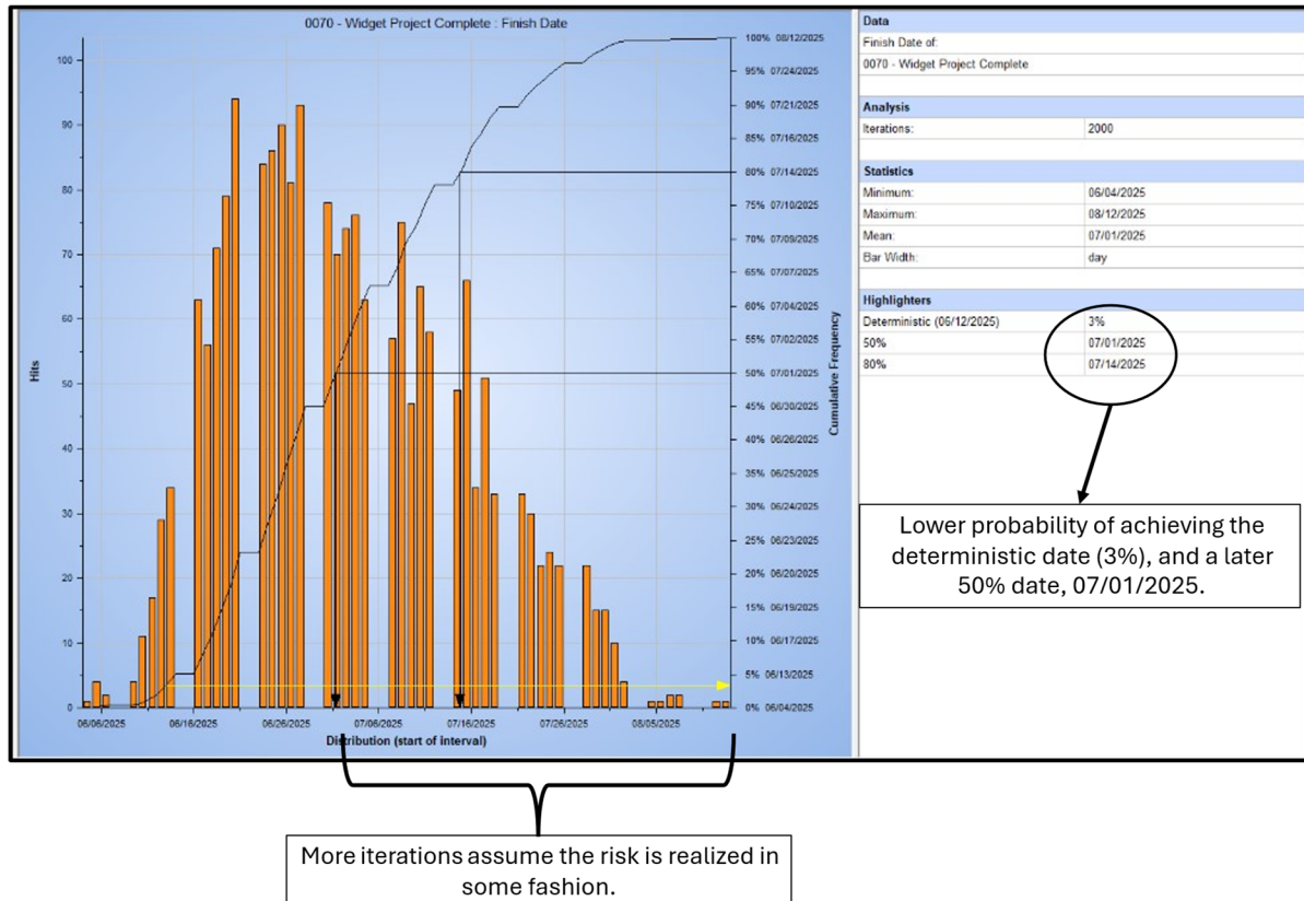
Figure 10.3.2-6 Example SRA Output – Inaccurate histogram results as a result of incorrectly modeling a discrete risk in a worst case duration estimate
