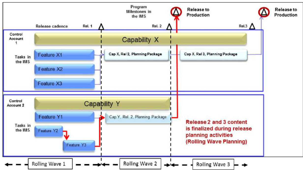
Figure 13.3-3: Modelling Rolling Waves in Agile
