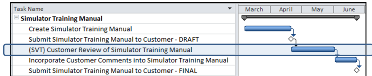
Figure 7.3-2 Example of the use of an SVT to capture Customer Review Time
