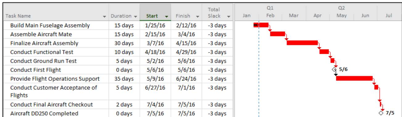
Figure 10.1-1 Example of a Program Critical Path
