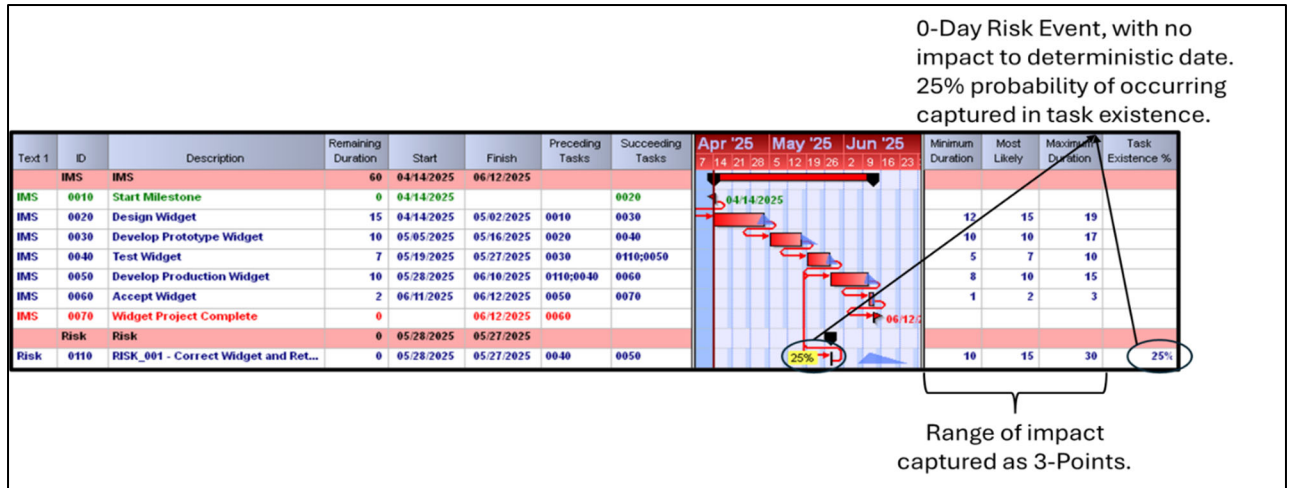
Figure 10.3.2-2 Example of the Risk Milestone Method for incorporation of discrete risks as an SRA input
