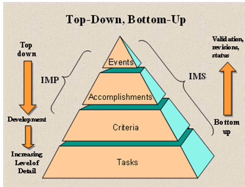
Figure 4.2-5 Top-Down, Bottom-up Methodology
