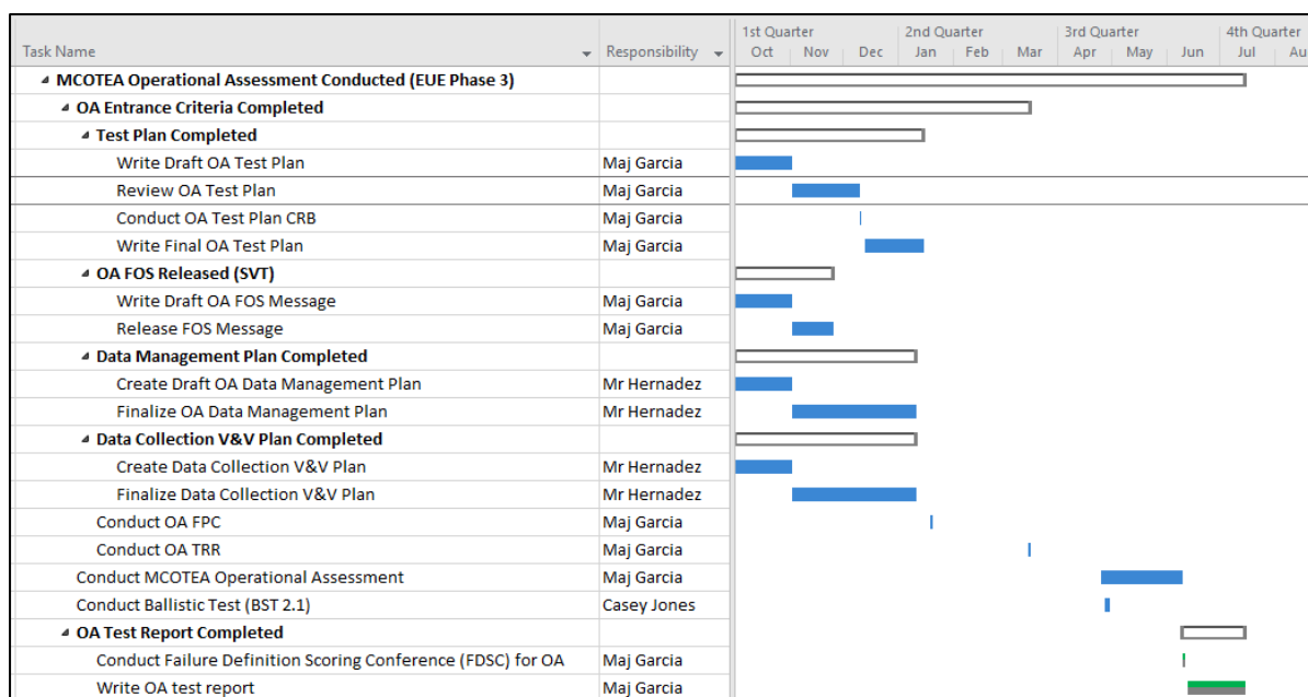
Figure 4.3-2 Example of an Integrated Master Schedule
