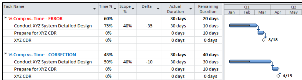
Figure 10.4.7-1 Results of identifying and adjusting duration to validate scope versus duration-based update
