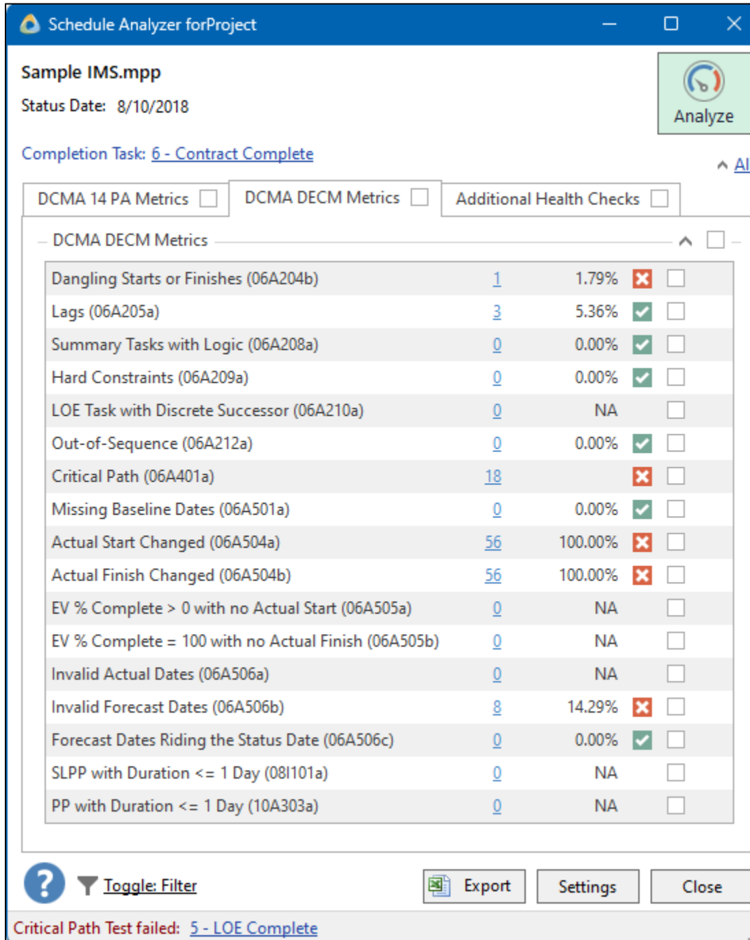
Figure 10.2-2 forProject Schedule Analyzer Example of Health Assessment Metrics
