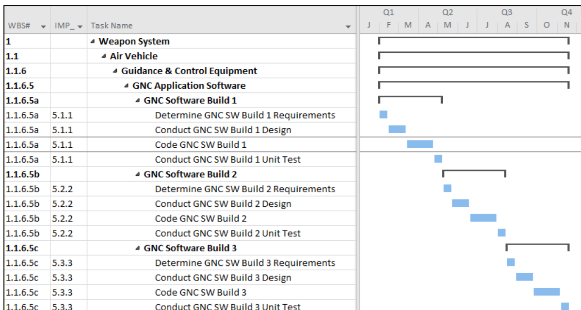
Figure 4.1-4 Detailed tasking structure based on the WBS architecture
