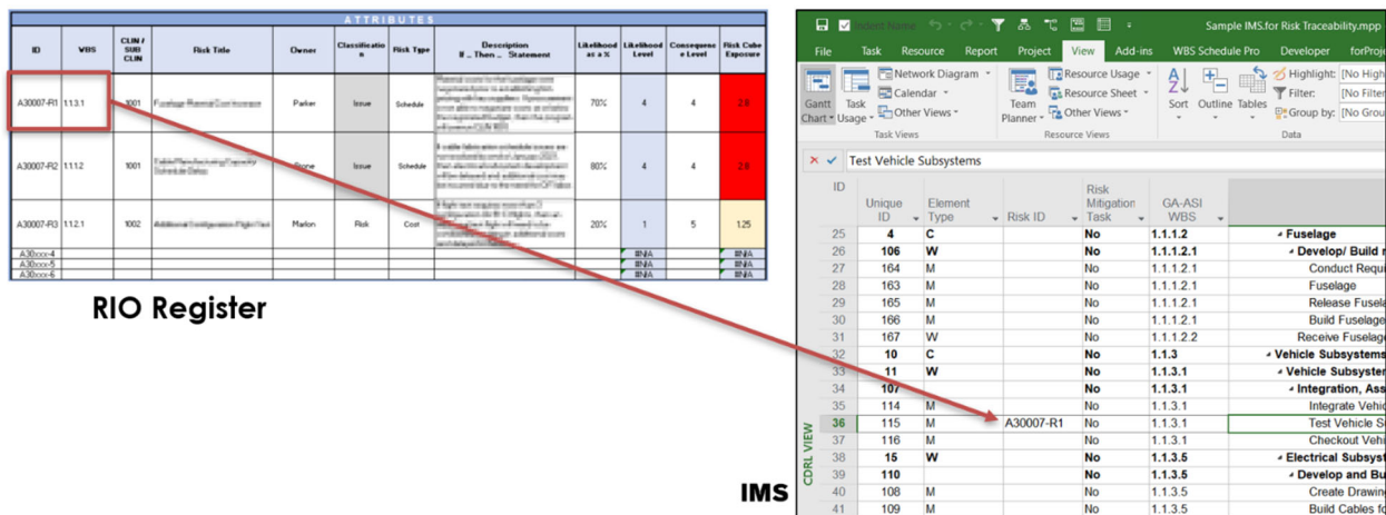
Figure 10.3.1-2 Integrating Risks and Opportunities into the IMS (Example only; not intended as a standard)
