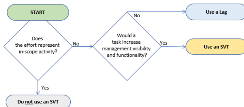
Figure 7.3-1 SVT Decision Tree
