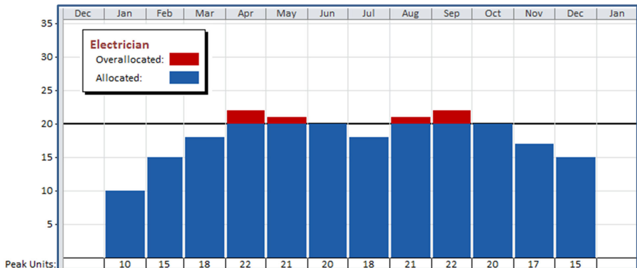
Figure 13.4-2 Example of Resource Histogram (after resource leveling is performed)
