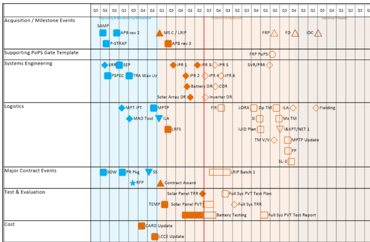
Figure 4.3-1 Example of a Summary Master Schedule
