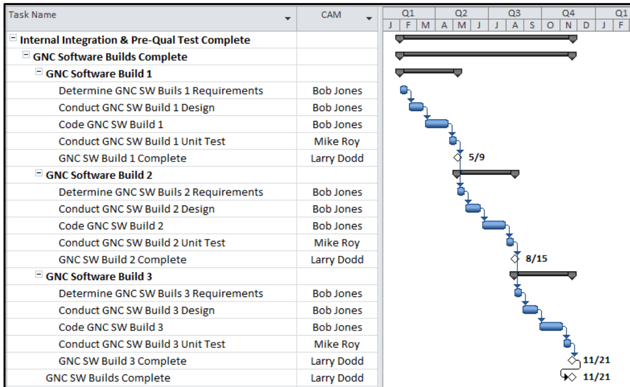
Figure 4.4-2 Example of Bottom-up Planning, supporting Top-down Planning from Figure 4.5-1 above
