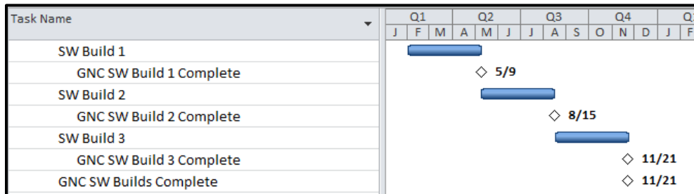
Figure 4.4-1 Top-Down Planning example demonstrating desired Periods of Performance
