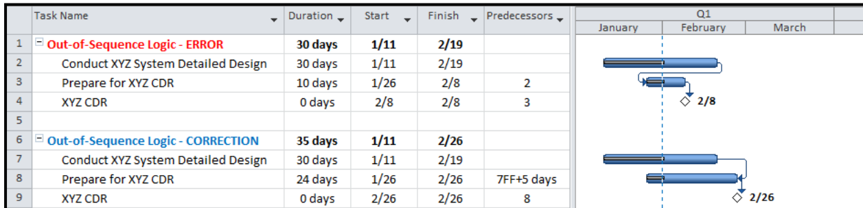
Figure 9.1.1-4 Impact of Out-of-Sequence Logic
