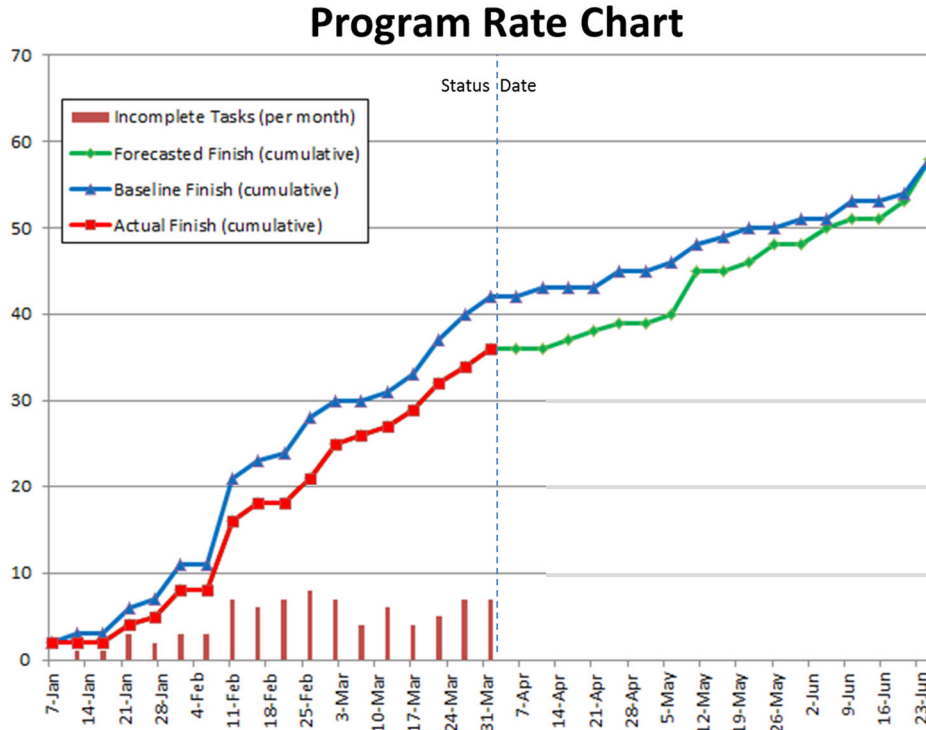
Figure 10.4.8-1 Program Rate Chart, showing actual data through March 31st, and ETC projections thereafter
