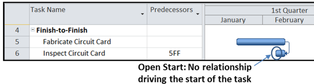
Figure 5.3-6 Example missing non-Finish-to-Finish Predecessor
