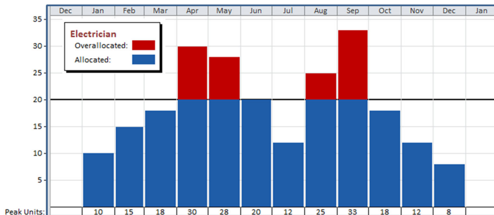
Figure 13.4-1 Example of Resource Histogram (prior to resource leveling)
